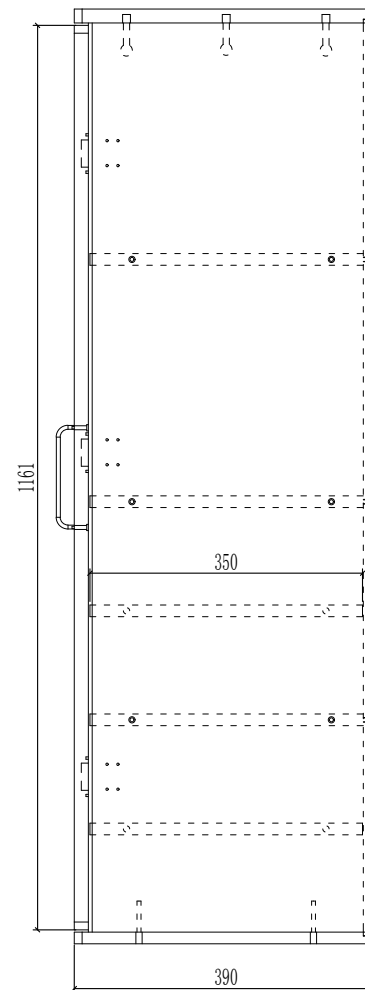
KB1-DG25228-30-F 6 Shelf Storage Cabinet A w/doors-H120cm
